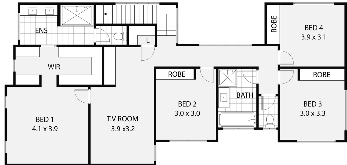
FIRST FLOOR
